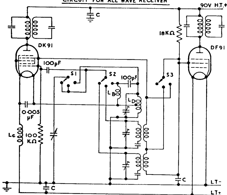
Fig. 4. All-wave Battery-operated Frequency Changer using DK91 Heptode
