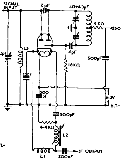
Fig. 6. U.H.F. Mains-operated Frequency Changer using EAC91 Diode-Triode
