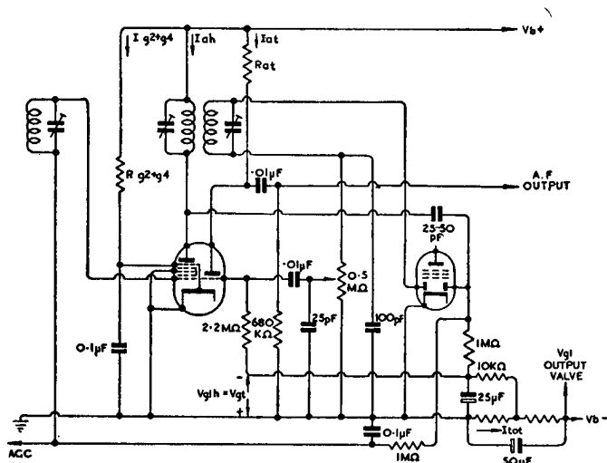
Fig. 9.—Circuit for triode-heptode as combined I.F. and A.F. amplifier.
